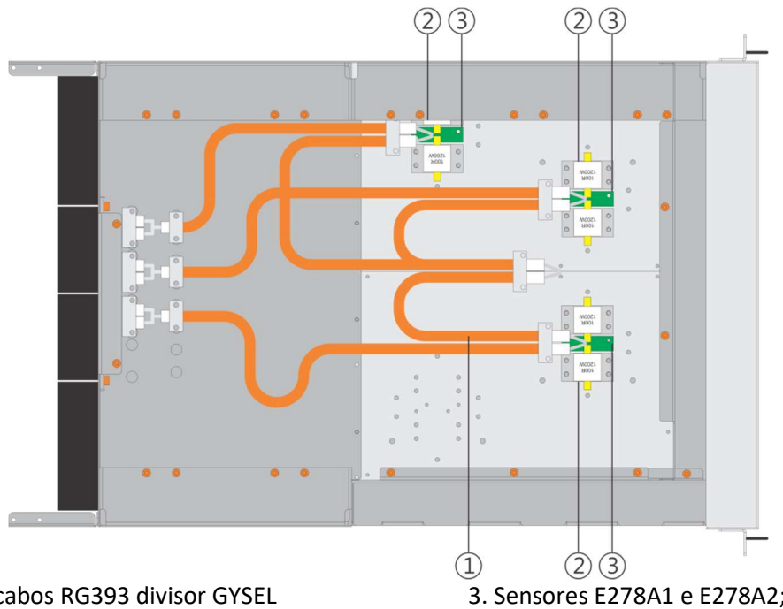
Figura 36: Vista superior DL1330S/E
